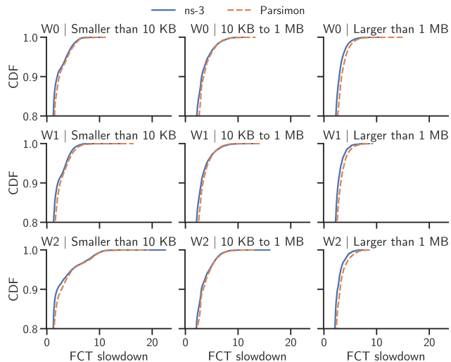
Figure 11. CDFs of FCT slowdown for ns-3 and Parsimon, bucketed by workload and flow size. Note the y-axes. When mixing workloads in a single simulation, Parsimon can accurately estimate performance distributions for individual workloads in addition to full-network aggregates.
