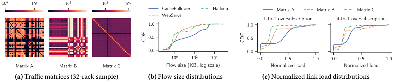
Figure 6. In the evaluation, we model workloads using data from Roy et al. 's study of Meta's data center network [28]. The traffic matrices in Fig. 6a are extracted from the accompanying dataset, and the flow size distributions in Fig. 6b are estimated from the published data. Lastly, for a given topology, the distribution of link loads depends on 1) the traffic matrix and 2) the degree of oversubscription. Fig. 6c shows the link loads induced by the matrices in Fig. 6a on two 32-rack topologies with different overprovisioning. The x-axis is normalized to the maximum link load.
