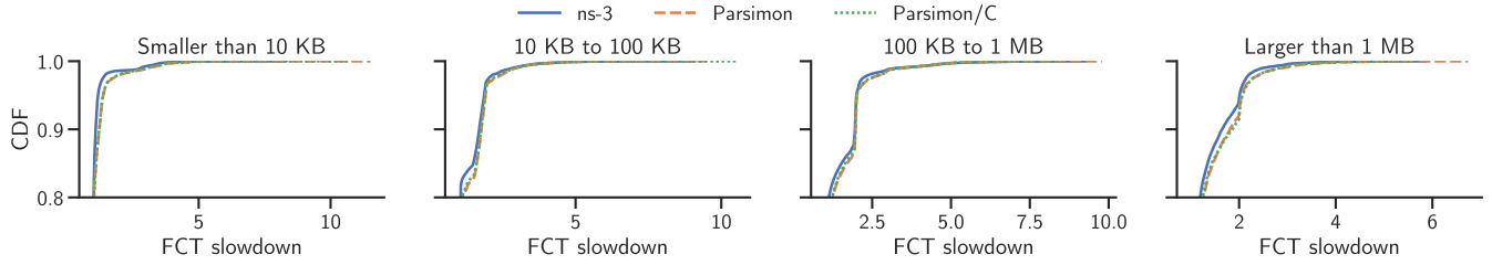
Figure 7. CDFs of FCT slowdown estimated by ns-3 and two Parsimon variants (note the y-axis). On a large network with 6,144 hosts, an industry traffic matrix (matrix B), and 2-to-1 oversubscription in the core, Parsimon’s latency estimates are similar to those produced by full-fidelity simulation. Table 2 shows the performance of each estimator.
