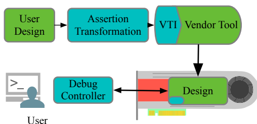
Figure 2. Design overview of Zoomie. Elements in blue denote Zoomie components.
